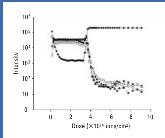
FIGURE 2. Secondary ion intensities (log scale) as a function of increasing SF_5^+ primary ion dose for PLA films doped with 5% theophylline.
